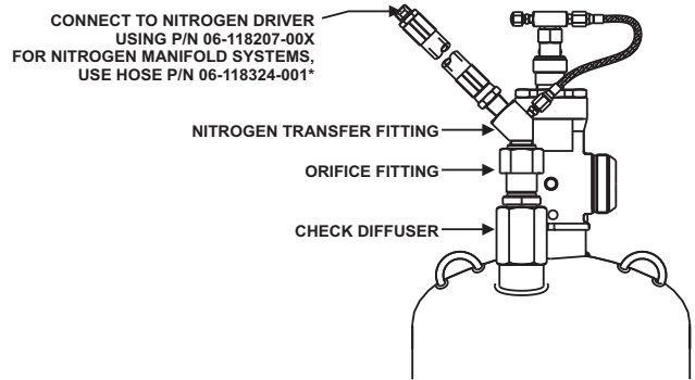
Cylinder and Valve Assembly with Assembled Actuation Components
